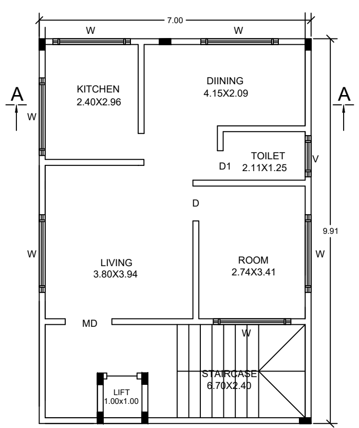
TYP:FIRST & SECOND FLOOR PLAN
