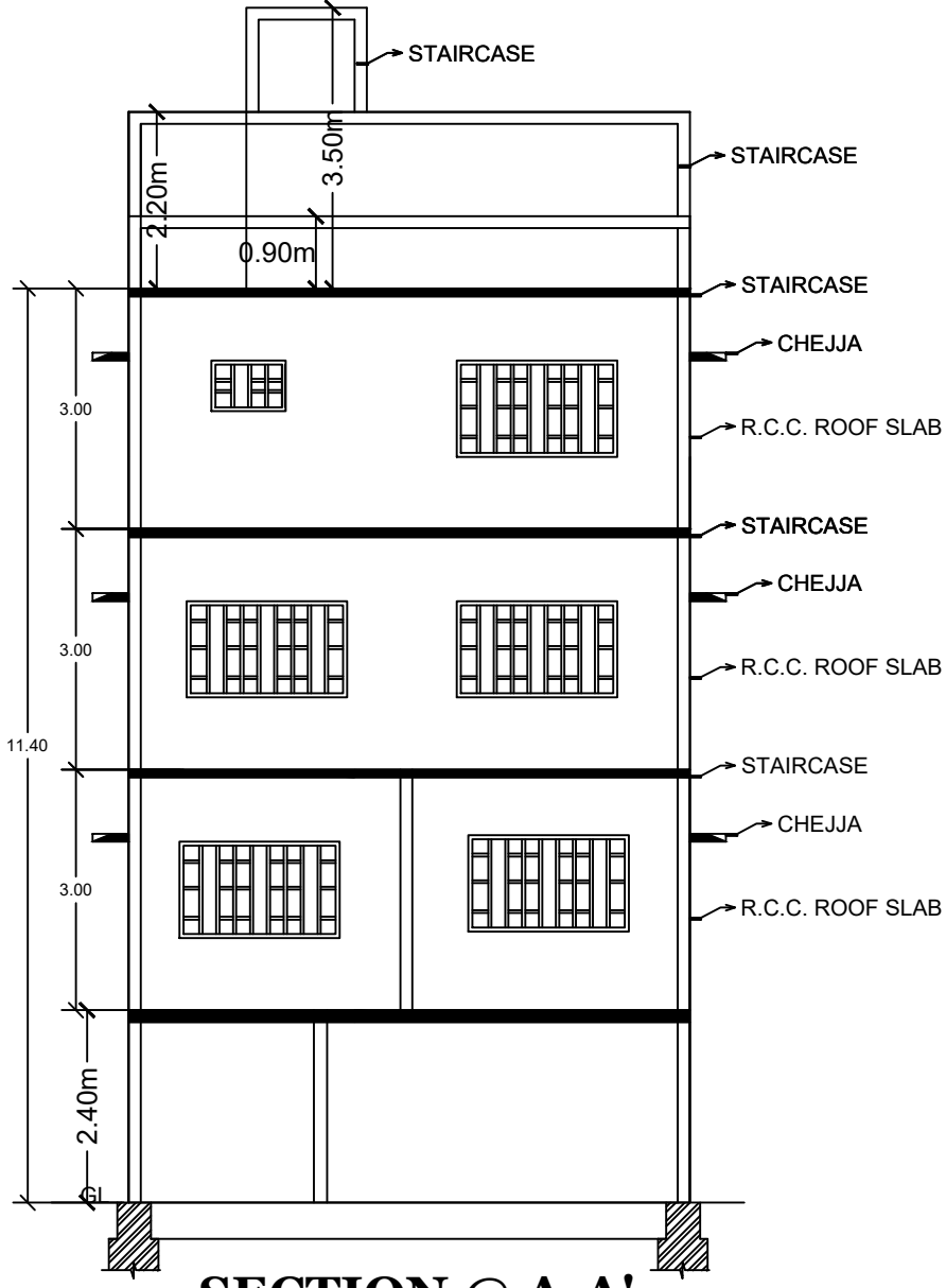
SECTION @ A-A'
